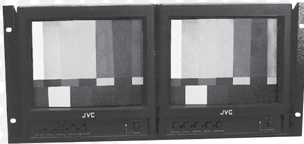
SS-5 5U Stationary Shelf with dual 9" JVC Monitors
