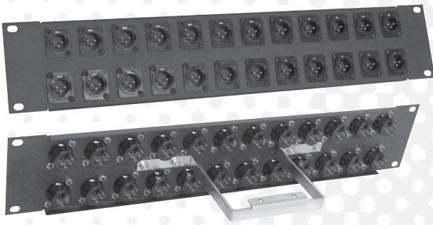
BOP-4 2U Breakout Panel, 24 XLR, Rear Cable Relief Bar
