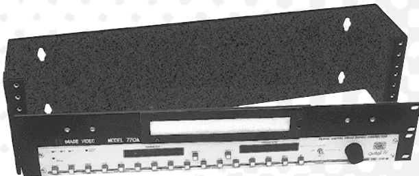
HWM-3 3 U Hinged Wall Mount Bracket with two control panels
